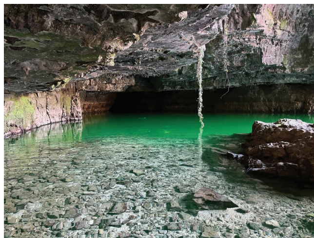
Fig. 4 - Oliero Covol dei Veci. Bright green water where the water is deep, here up to 15 m; in the foreground the depth is around 0.5 – 1 m and the color is less visible. Photo 30 th November around 13:45 pm almost at the maximum concentration 6.7 \mu\text{g/L} registered.
