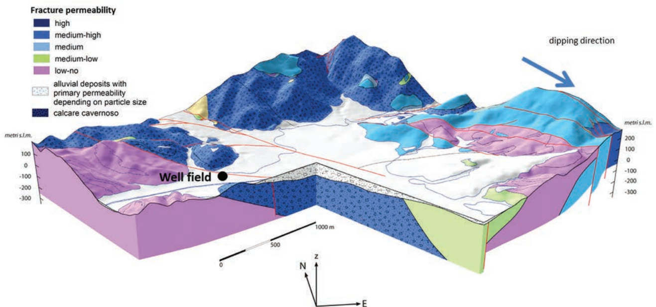
Fig. 2 - 3D reconstruction of hydrostructure.
