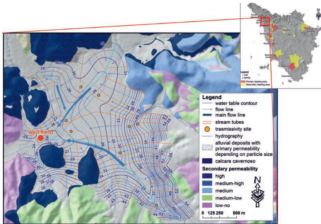
Fig. 3 - Hydrogeological map and water table contours (m a.s.l. – June 2012). Water level data were collected after a period without significant rainfall.
